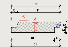
Varius 20 x 91
