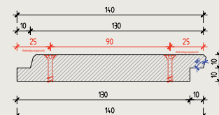
Varius 20 x 140
